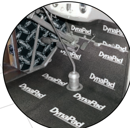
Firewall
